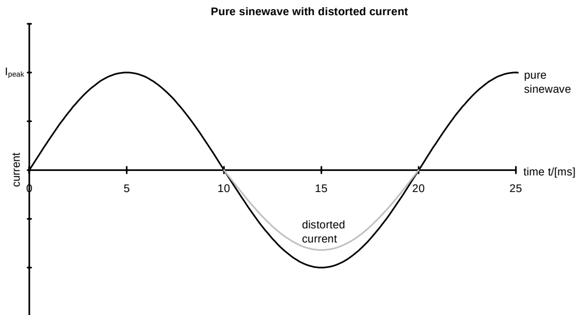
Figure 1 Current with an asymmetrical wave shape.
