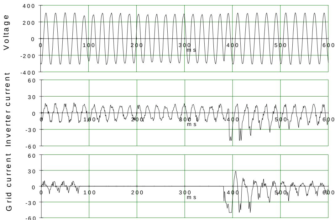
Fig. 3 Re-closing test
