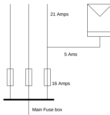
Figure 2 Connection of an AC Module to a normal feeder
