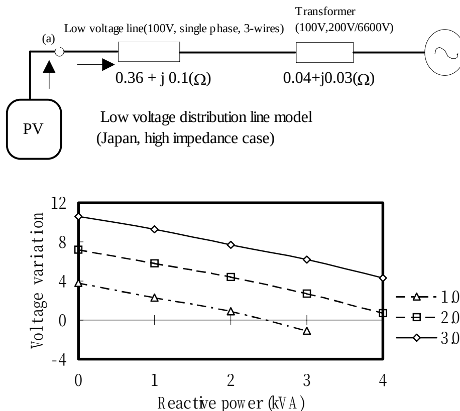
Figure 2 A calculation result on suppression of voltage rise by reactive power control of PV system. Parameter; Real power of PV system
