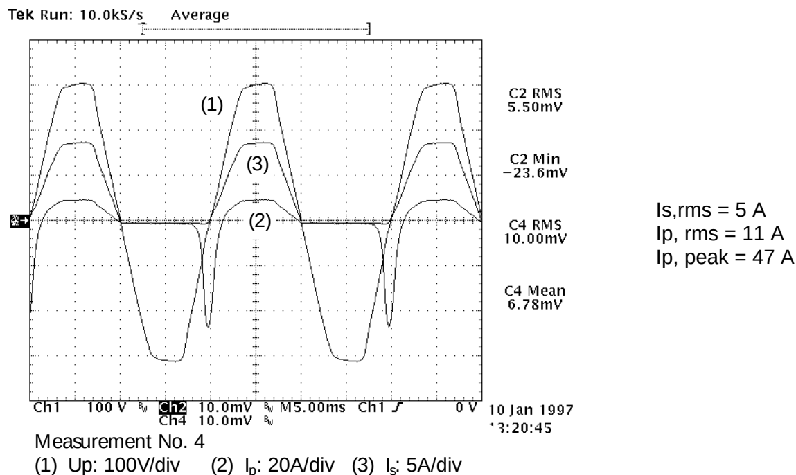
Figure3 Line voltage U_p , (1), primary current I_p , (2), and secondary current, I_s , (3) for a pulsed dc load.
