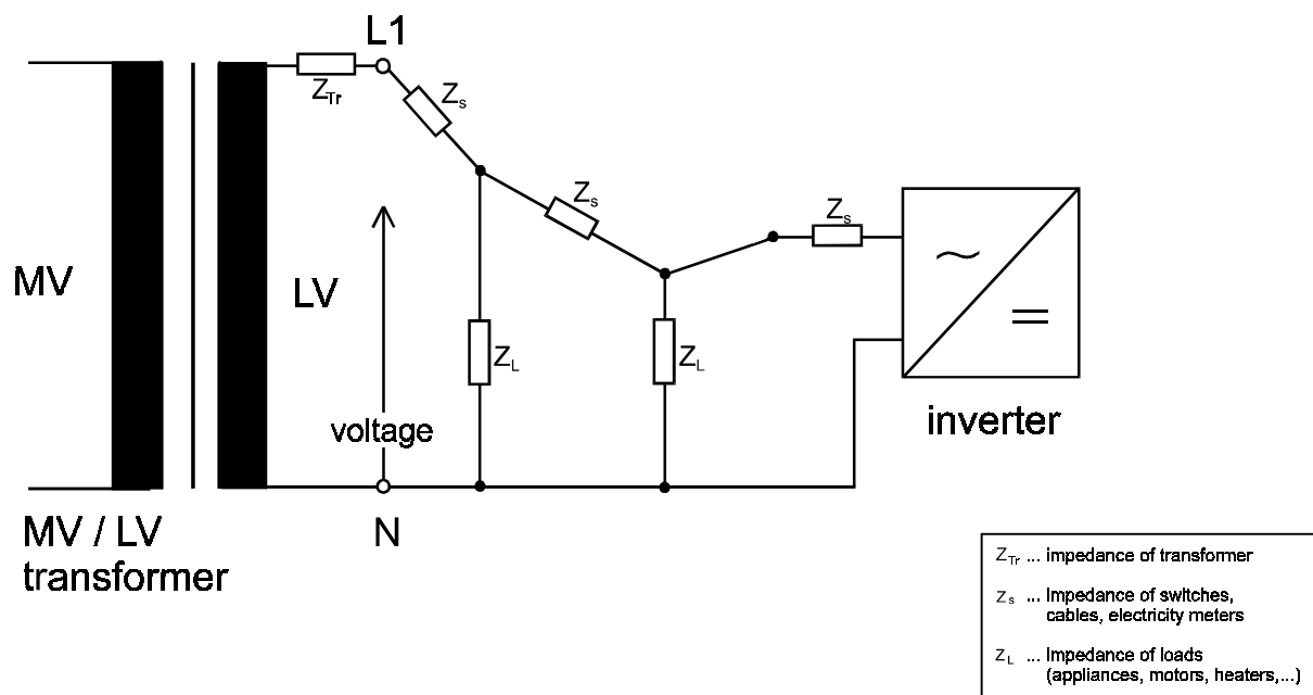
Figure 1 Typical situation in a low-voltage distribution line with one independent power producer.
