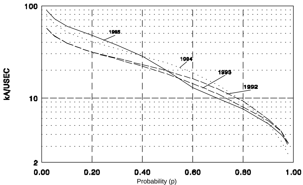
Figure 4 Probability of the di/dt of lightning current
