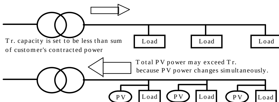
Figure 3 Effect of reverse power flow on transformer capacity
