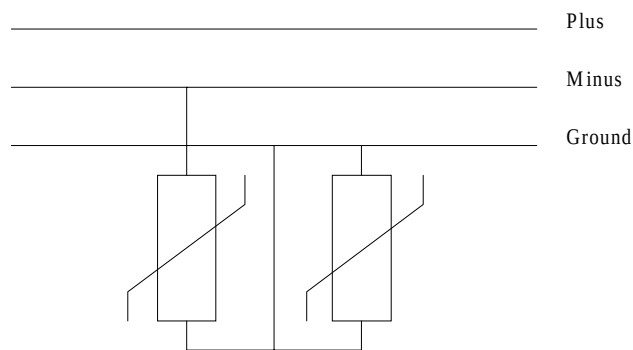
Figure 9 Connection of surge arrestors
