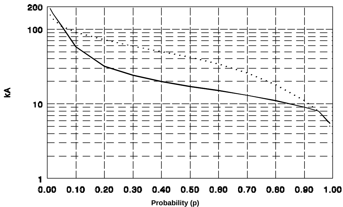
Figure 3 Probability of the peak value of a lightning strike
