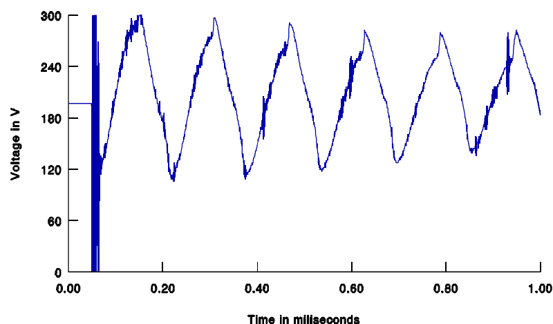
Figure 8 Result of lightning induced voltage in an array
