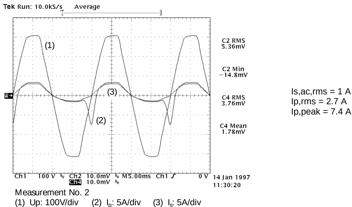
Figure 5 Line voltage U_p , (1), primary current I_p , (2), and secondary current, I_s , (3) for a dc current of 1 A and an ac load of 1 A.
