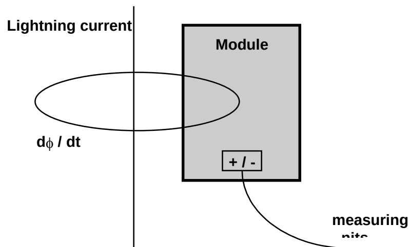
Figure 6 Schematic overview of measuring of the induced voltage in a PV module
