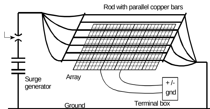
Figure 7 Schematic overview of test set-up for lightning induced voltage in an array of PV modules. Two strings with each 18 modules connected in series.
