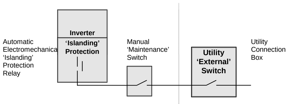
Figure 11.1 External Disconnect Methods
