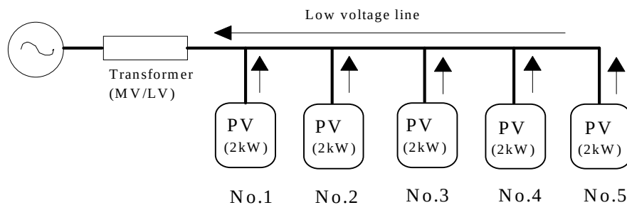
(a) State of reverse power flow
