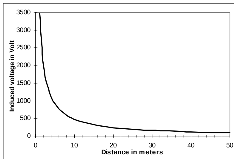
Figure 5 Induced voltage in a loop of 1 \text{ m}^2 versus the distance between the loop and the lightning current
