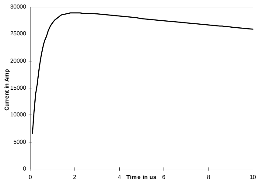
Figure 2 Typical lightning current
