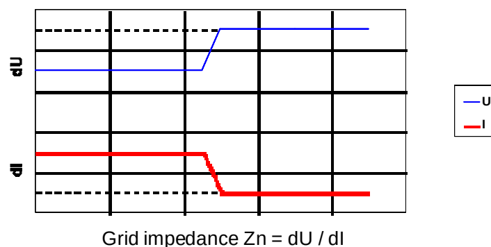
Figure 2 Grid impedance calculation by current and voltage jumps
