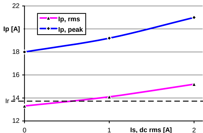
Figure 8 Primary current versus secondary dc component; constant ac load of 12 A
