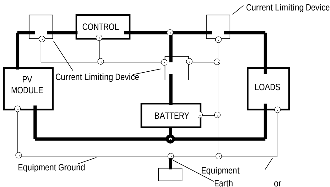
Figure 2. PV System with Equipment Grounding Only
