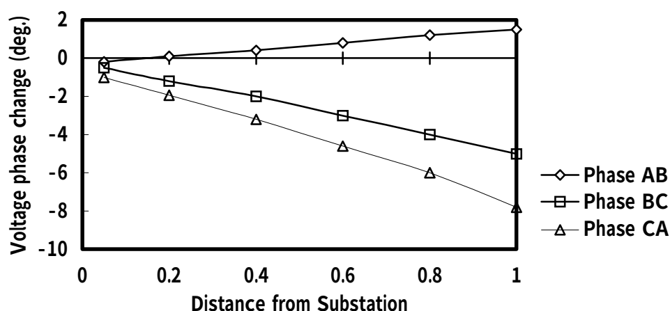
Figure 4 A calculation result on voltage phase change in case of short circuit fault with high resistance - 2 phase fault on MV(=6.6kV) line of Japan - Fault point ; end of line(3.8km from substation)
