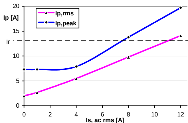
Figure 6 Primary current versus ac load; fixed dc component of 1 A.
