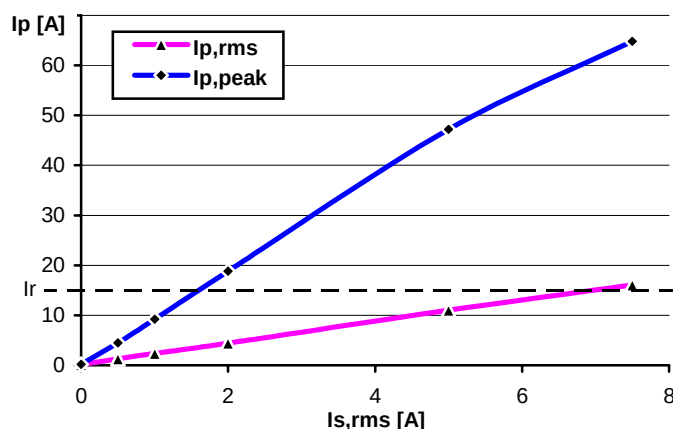
Figure 4 Primary current versus secondary dc current; no ac load. I_r indicates the rated primary current. It needs a high dc component to exceed the rated current I_r .
