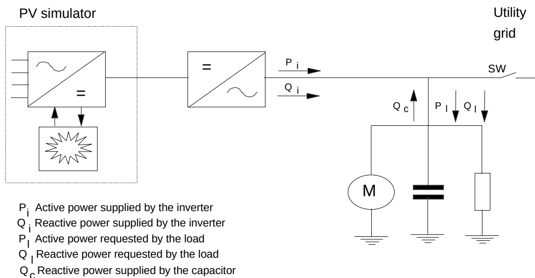
Fig. 2 ENEL test circuit
