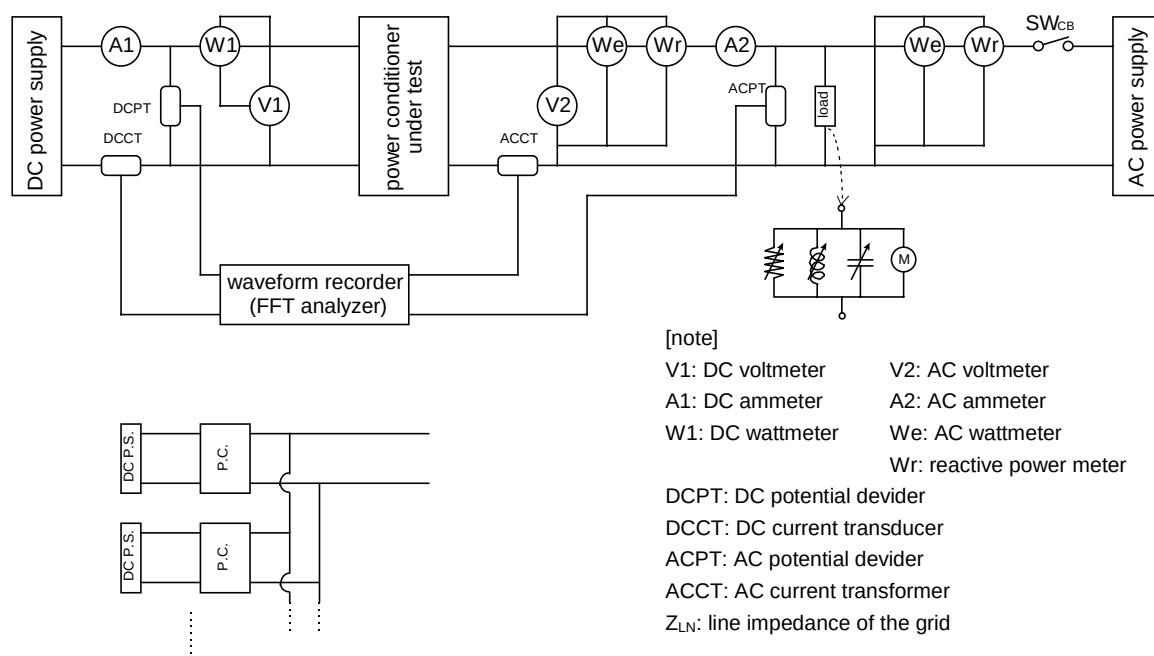
Figure 1 Test circuit for utility connected power conditioners
