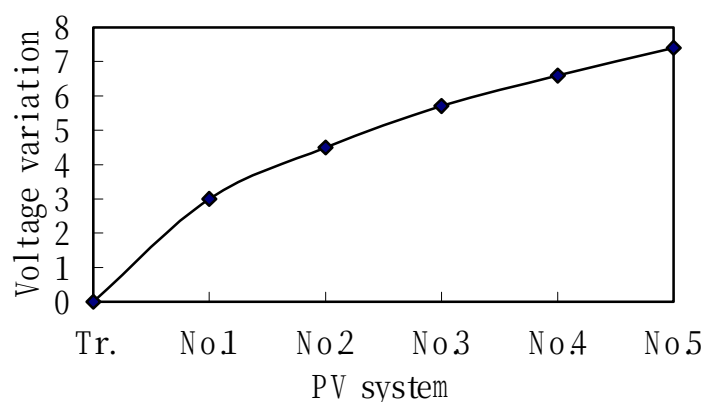
(a) State of reverse power flow
