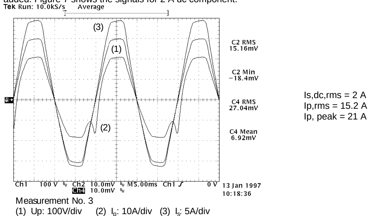
Figure 7 Line voltage U_p , (1), primary current I_p , (2), and secondary current, I_s , (3) for an ac load of 12 A and 2 A dc load. The current peak from saturation is below the regular peak load current.
