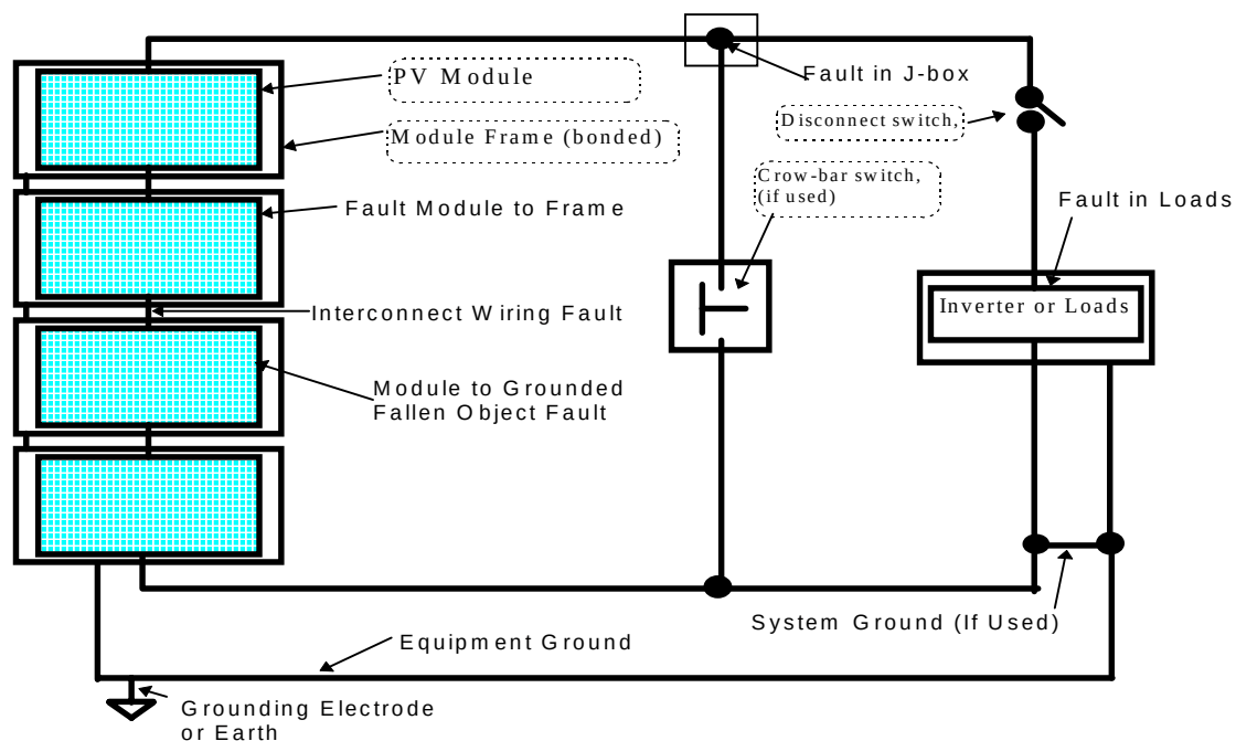
Figure 1 Typical PV system showing locations of possible ground faults.
