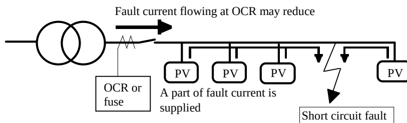
Figure 5 Fault current flow under short circuit fault of distribution line
