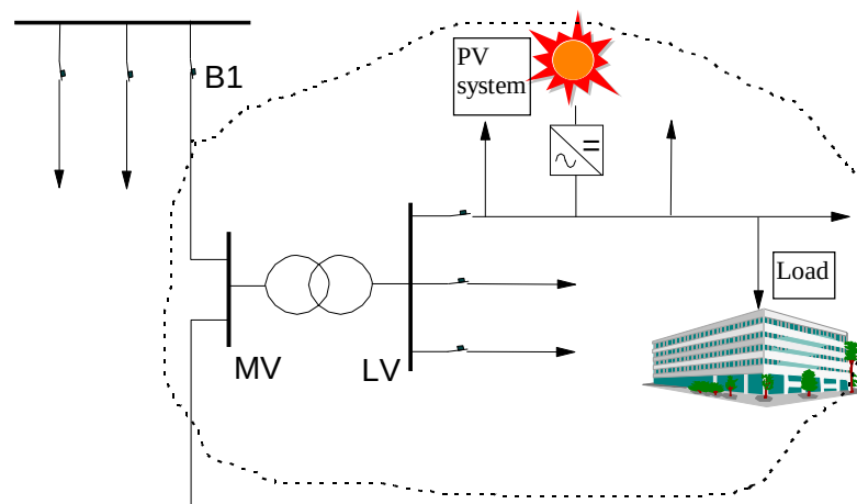
Figure 1 MV network re-closing affecting PV system connected to the LV network
