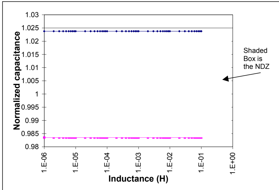
Figure 2a. Mapping of the NDZ of the Over/underfrequency Protective Devices in the RLC Load Space. (Note that for the frequency devices only, the load resistance has no effect, and thus only inductance and capacitance appear in the figure.)
