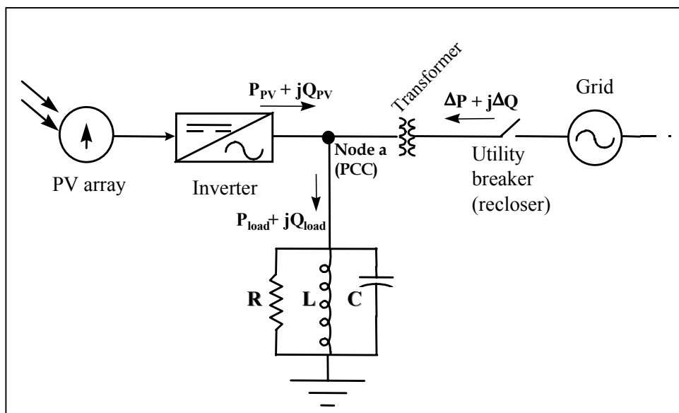
Figure 1. PV System/Utility Feeder Configuration Showing Definitions of Power Flows and Terms
