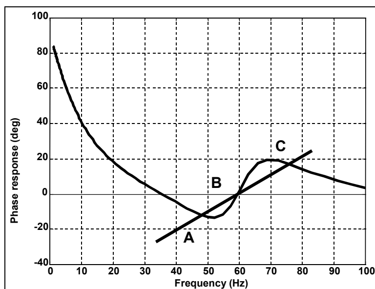
Figure 5. Plot of the Current-Voltage Phase Angle vs. Frequency Characteristic of an Inverter Utilizing the SMS Islanding Prevention Method [7]
