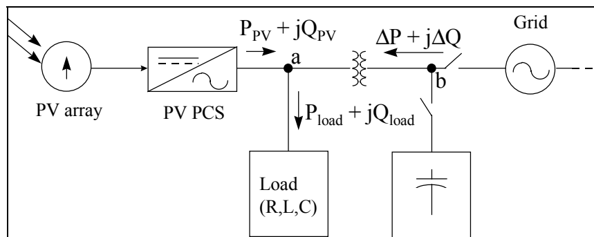
Figure 9. The Impedance Insertion Method Shown Implemented with a Capacitor Bank
