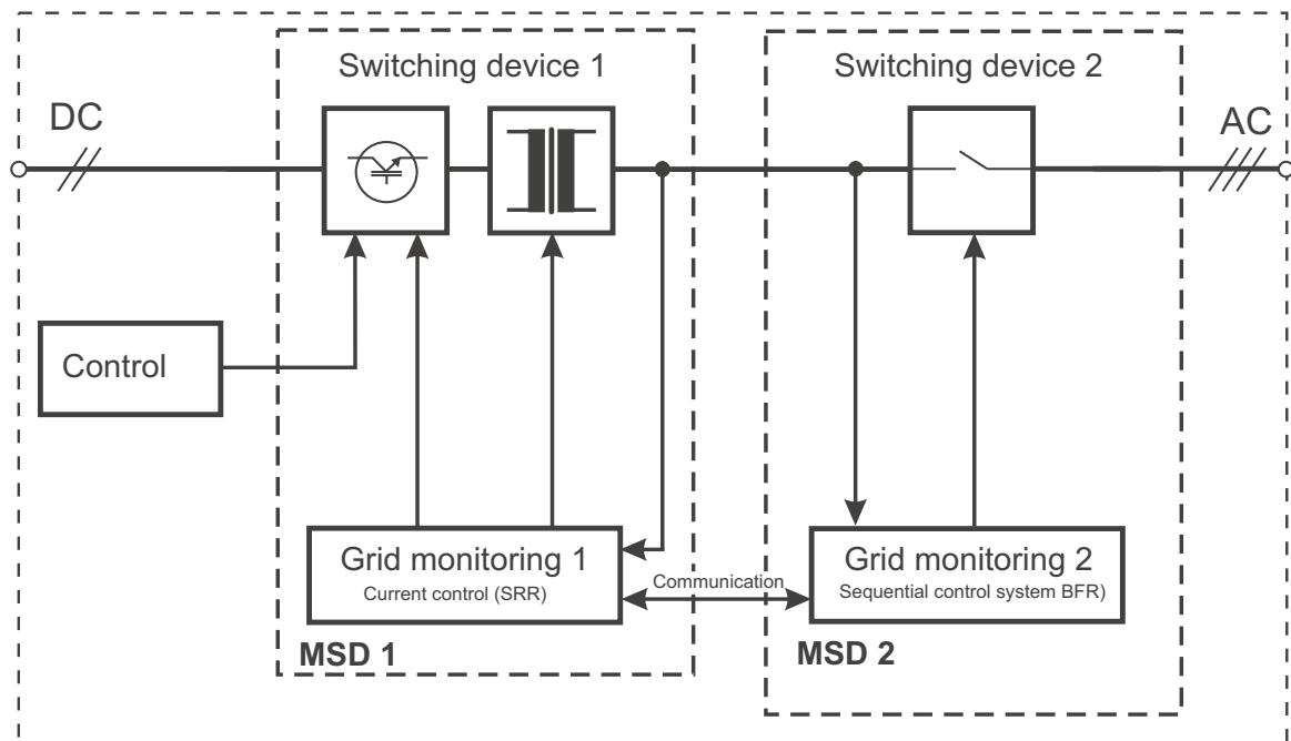
Figure 8. Design of an Automatic Disconnection Device According to DIN-VDE-0126
