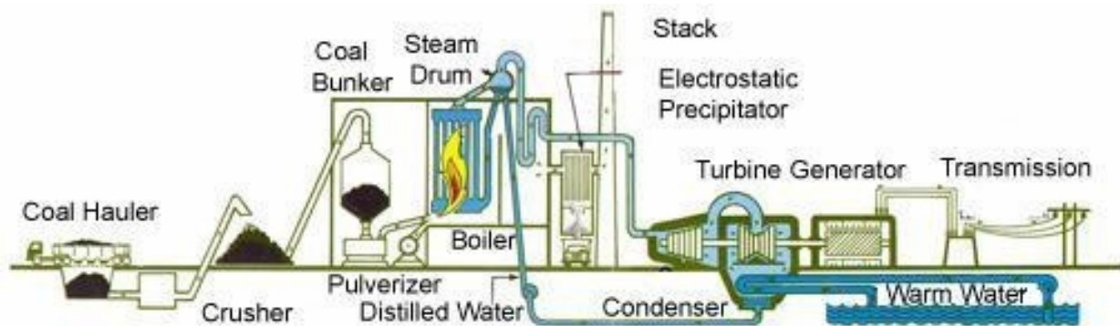
Figure 7. Stages of a Coal Fired Thermal Plant
